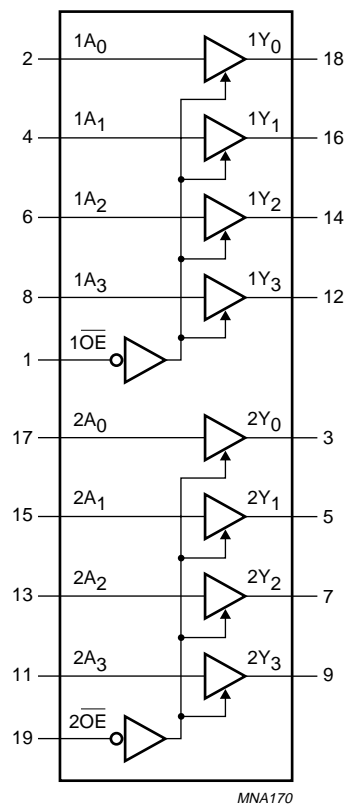
Fig.3 Logic diagram.
