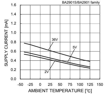
Fig. 66 Supply Current - Ambient Temperature
