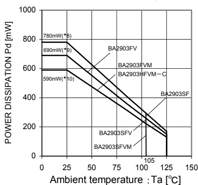
(c)BA2903 family
