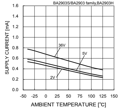
Fig. 43 Supply Current - Ambient Temperature
