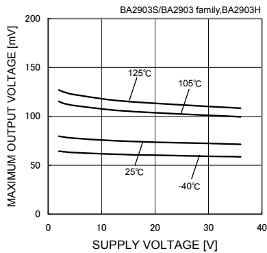
Fig. 44 Maximum Output Voltage - Supply Voltage (IOL=4mA)
