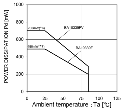
(b)BA10339 family
