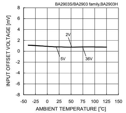
Fig. 49 Input Offset Voltage - Ambient Temperature
