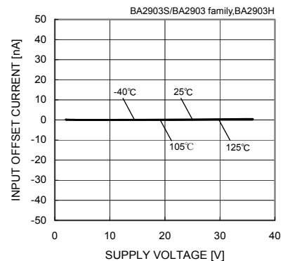
Fig. 52 Input Offset Current - Supply Voltage
