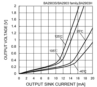
Fig. 46 Output Voltage - Output Sink Current (VCC=5V)
