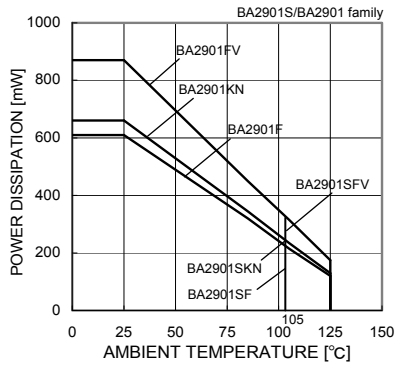
Fig. 64 Derating Curve
