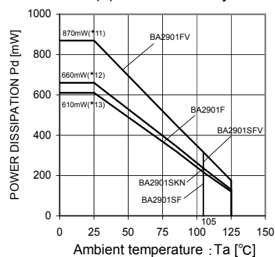
(d)BA2901 family
