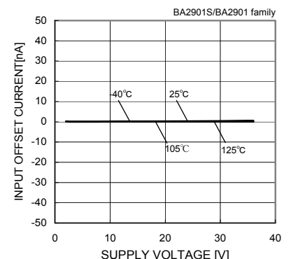
Fig. 75 Input Offset Current - Supply Voltage
