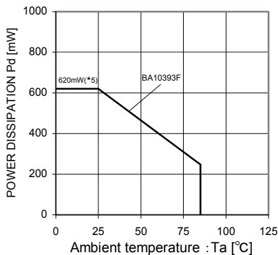
(a)BA10393 family
