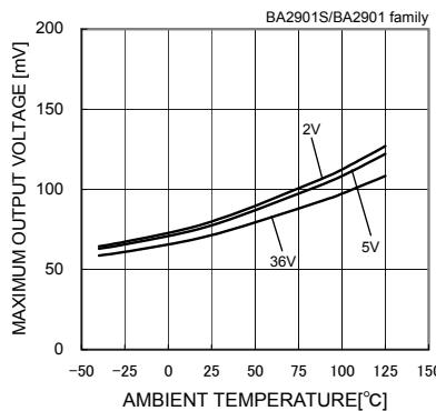
Fig. 68 Maximum Output Voltage - Ambient Temperature (IOL=4[mA])
