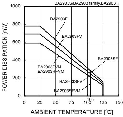
Fig. 41 Derating Curve
