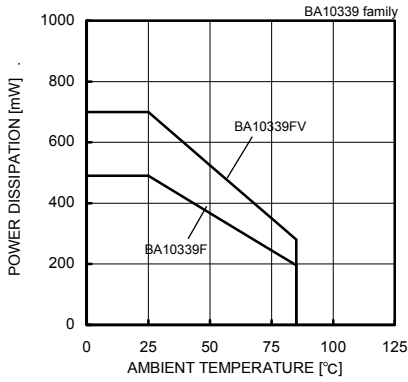
Fig. 21 Derating Curve
