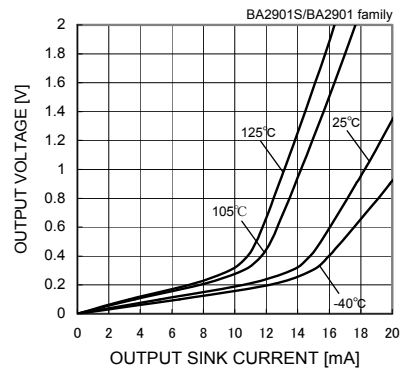
Fig. 69 Output Voltage - Output Sink Current (VCC=5[V])
