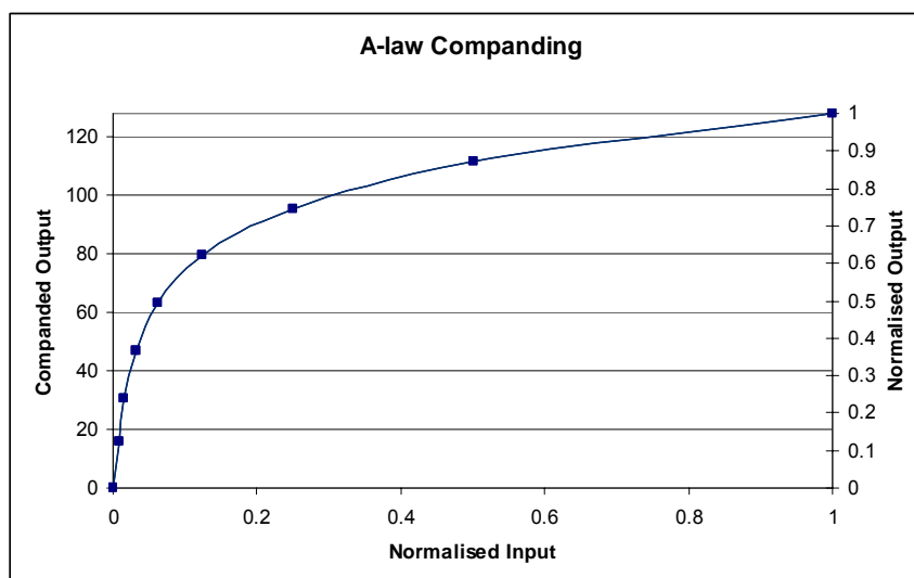
Figure 32 A-Law Companding
