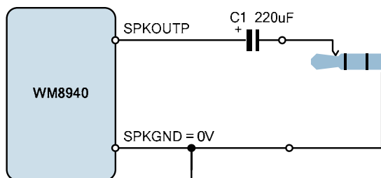
Headphone Output using DC Blocking Capacitors:
