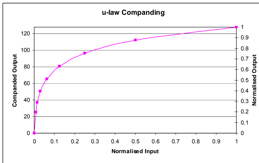
Figure 31 u-Law Companding
