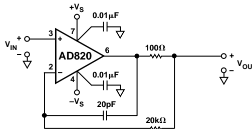
Figure 42. Extending Unity Gain Follower Capacitive Load Capability Beyond 350 pF
