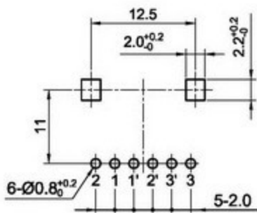
P.C.B. mounting hole detail
