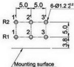
P.C.B mounting hole detail
