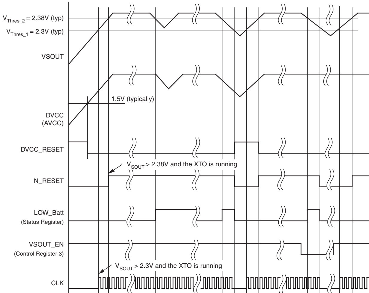
Figure 7-3. Reset Timing
