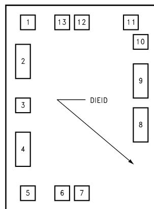
Figure 5. Die Layout (B - Step)
