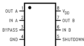
Figure 1. Top View Order Number LM4880M or LM4880N See NS Package Number M08A for SO or NS Package Number N08E for DIP
