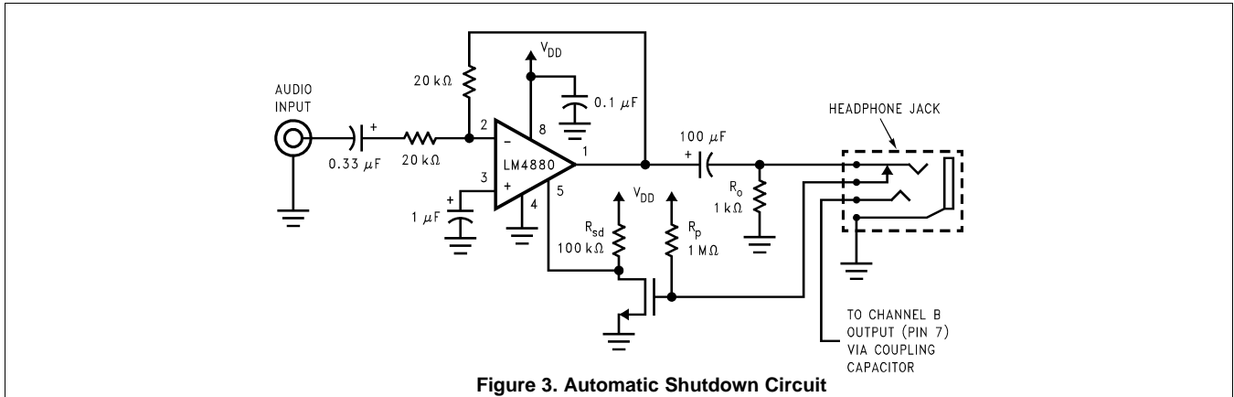
Figure 3. Automatic Shutdown Circuit
