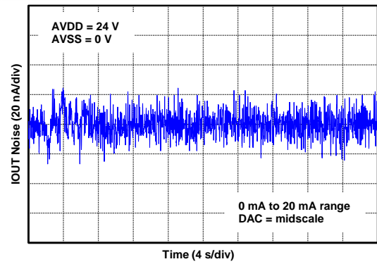
Figure 79. IOOUT PEAK-TO-PEAK NOISE vs TIME (0.1 Hz to 10 Hz)
