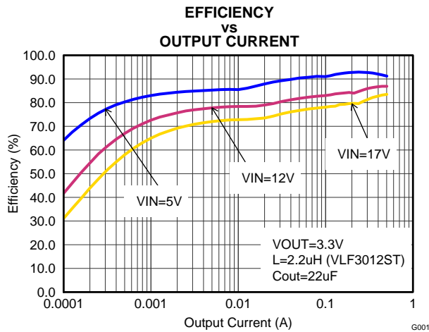
Figure 7. Vout=3.3V
