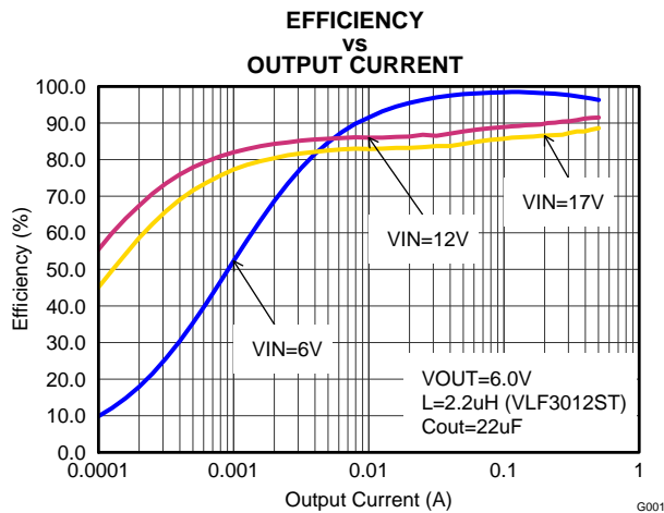
Figure 5. Vout=6V
