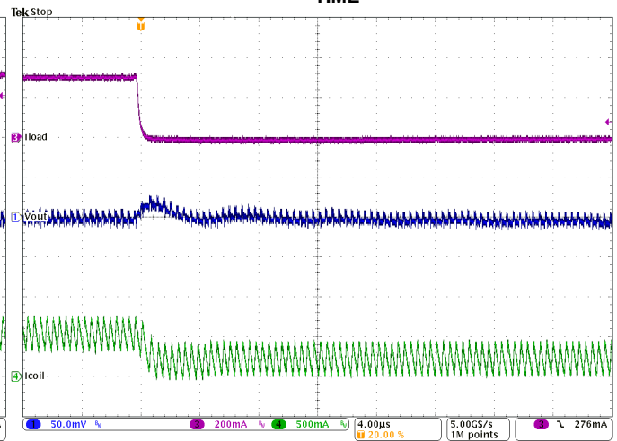
Figure 28. Load Transient Response in PWM Mode (200mA to 500mA), falling edge
