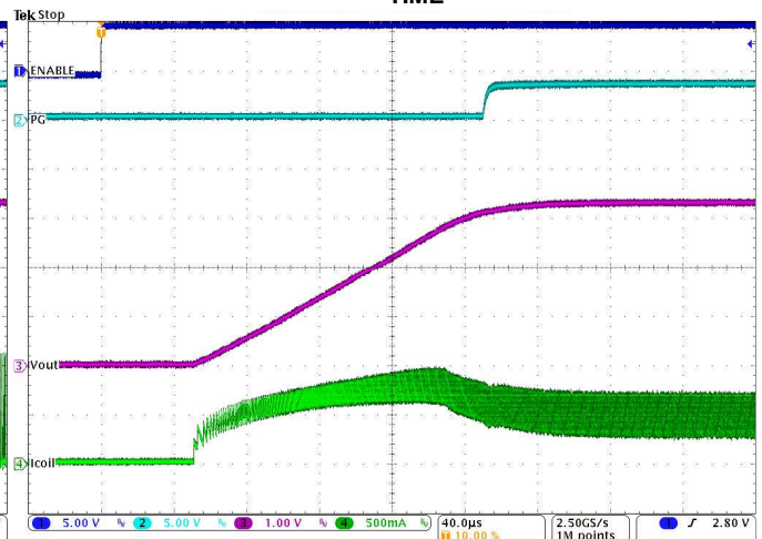
Figure 30. Startup with Iout=500mA
