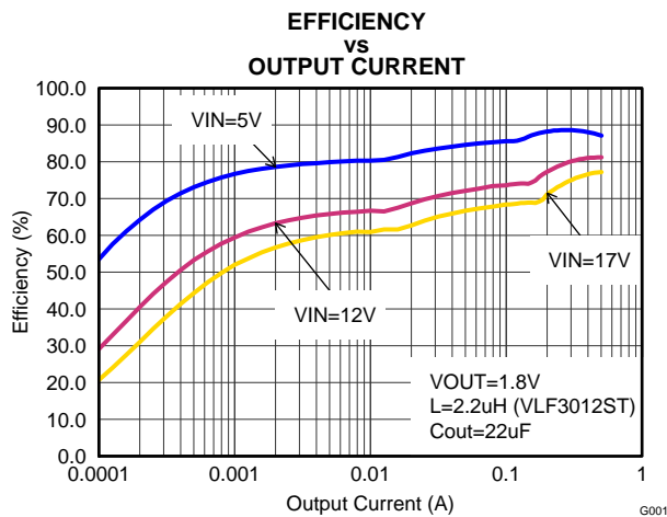
Figure 9. Vout=1.8V
