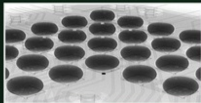
BGA 焊锡点饱满
