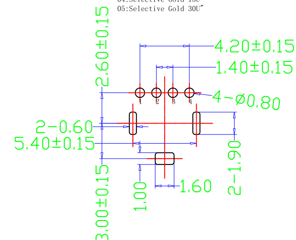
RECOMMENDED PCB LAYOUT GENERAL TOLERANCES: ±0.05
