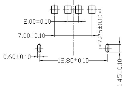
FRONT EDGE OF CONNECTOR PCB LAYOUT
