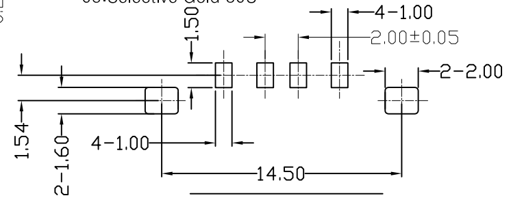
FRONT EDGE OF CONNECTOR PCB LAYOUT
