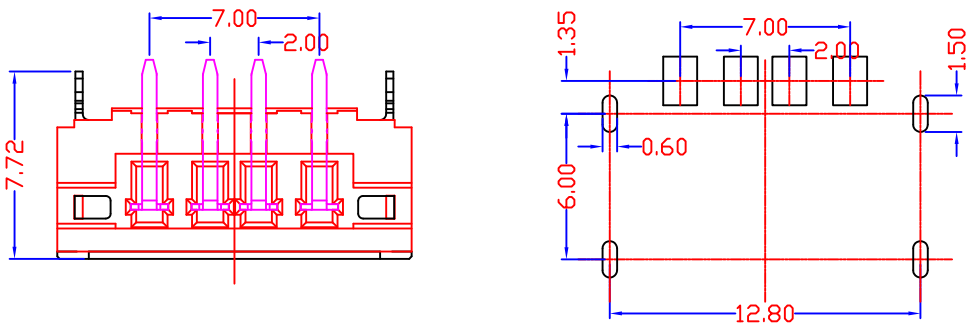
PCB HOLES
