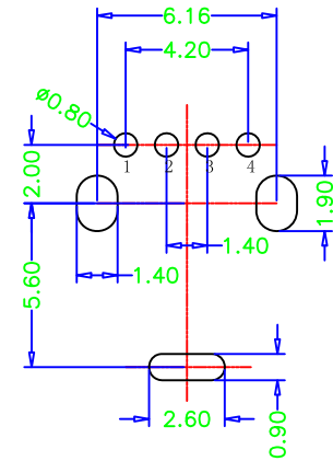
RECOMMENDED PCB LAYOUT GENERAL TOLERANCES: ±0.05
