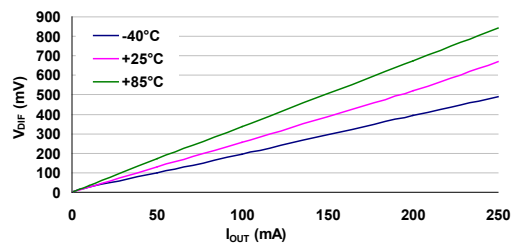
Dropout Voltage: HT7350-1
