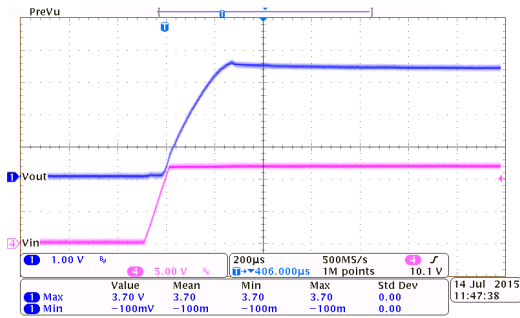
Power On Response: HT7333-1 ( I_{OUT}=0mA , T_{RISE}=0.1ms )
