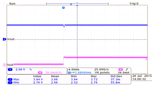
Load Transient Response: HT7333-1 ( V_{IN}=5.3V , I_{OUT}=0mA to 40mA )
