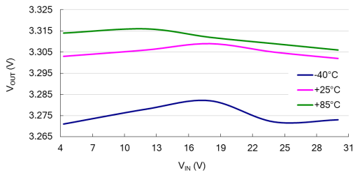
Line Regulation: HT7333-1 ( I_{OUT}=10mA )
