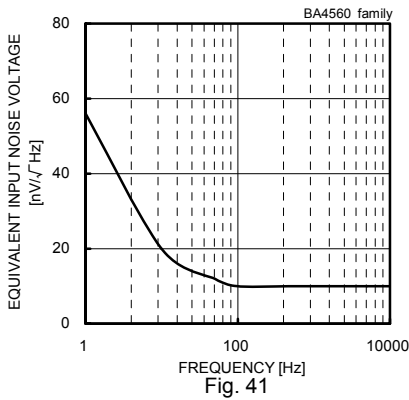
Fig. 41 Equivalent Input Noise Voltage – Frequency ( V_{CC}/V_{EE}=+15[V]/-15[V] , R_s=100[\Omega] , T_a=25[^\circ C] )
