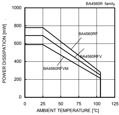
Fig. 67 Derating Curve
