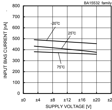
Fig. 165 Input Bias Current - Supply Voltage (Vicm=0[V], Vout=0[V])
