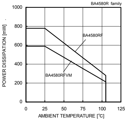
Fig. 89 Derating Curve
