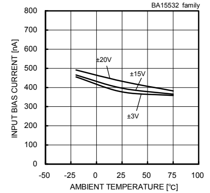
Fig. 166 Input Bias Current - Ambient Temperature (Vicm=0[V], Vout=0[V])
