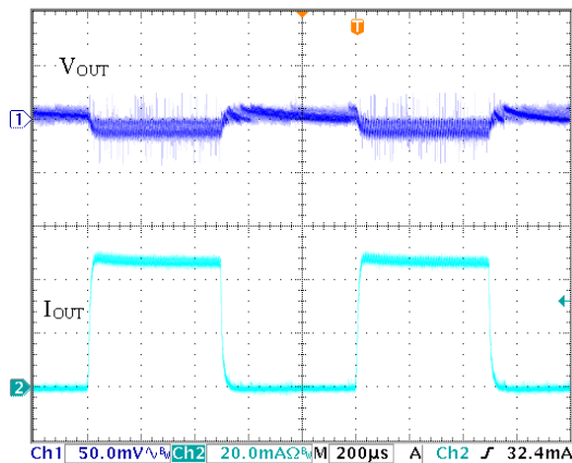
Fig 43. HT7722S Load Transient Response (L= 10µH, C IN = C OUT = 10µF, V IN = 1.32V)
