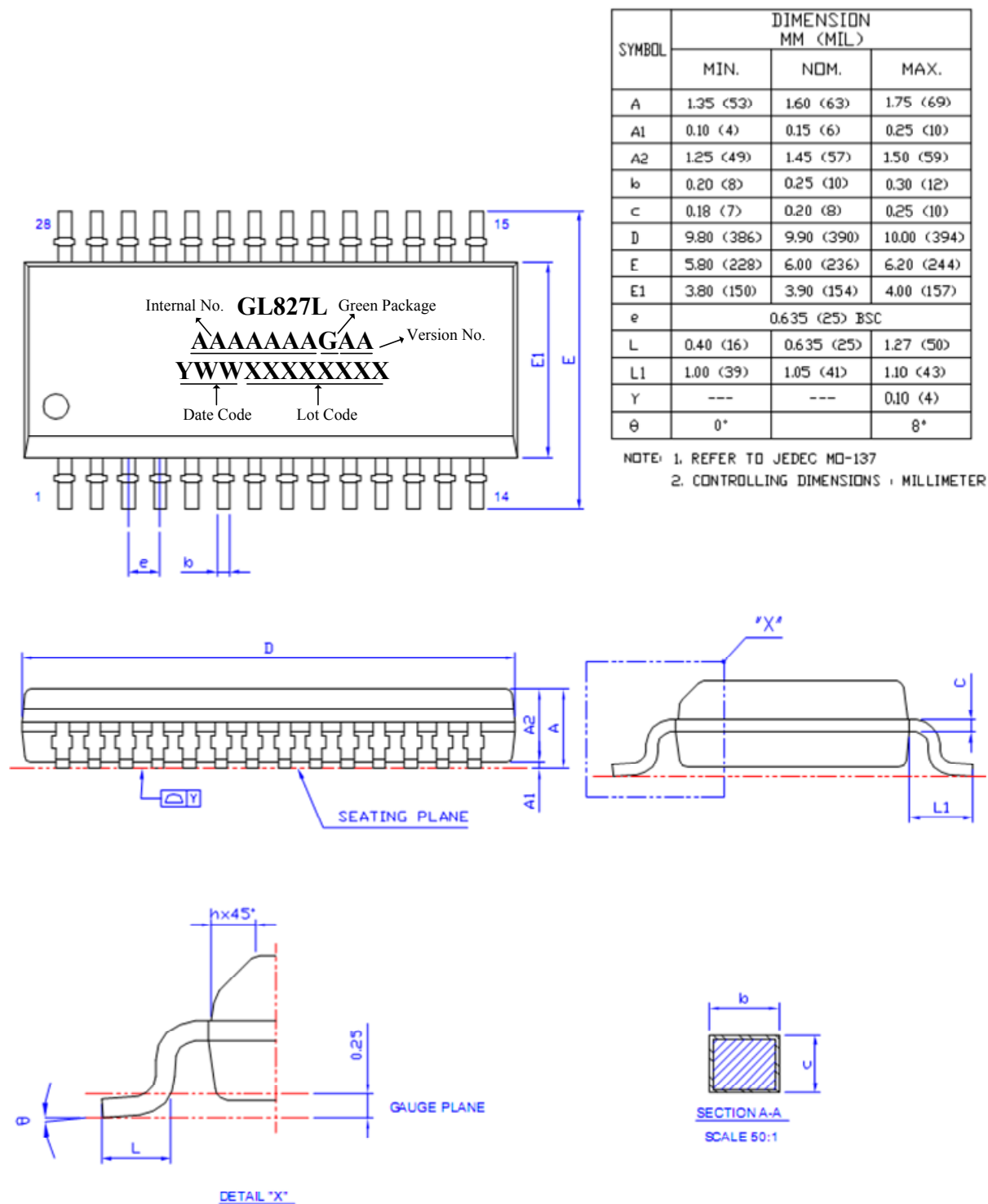
Figure 7.1 - GL827L 28 Pin SSOP Package
