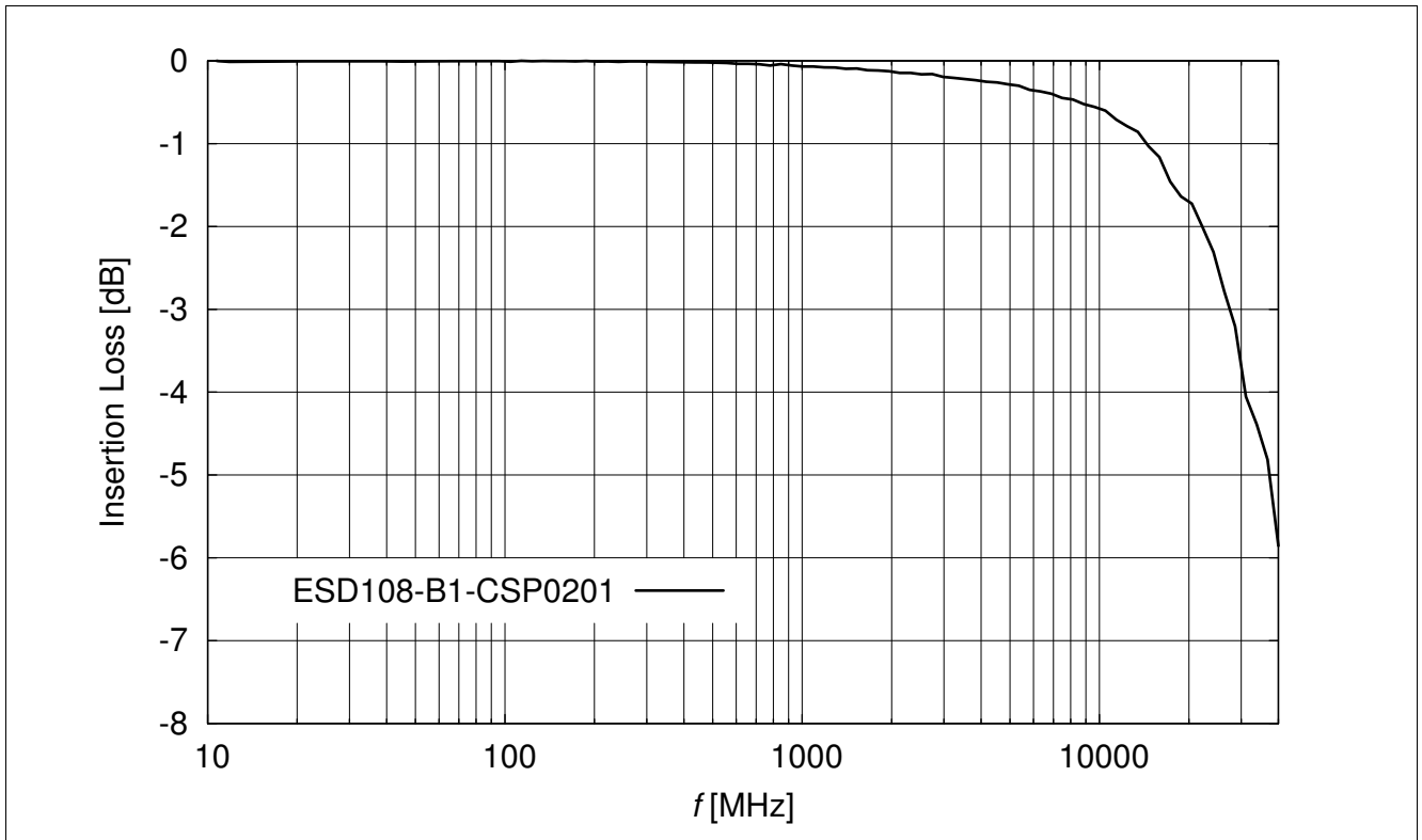
Figure 4-10 Insertion loss vs. frequency in a 50 \Omega system
