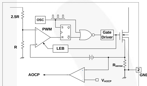
Figure 35. AOCP Block
