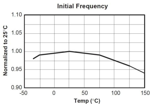
Figure 9. Initial Frequency
