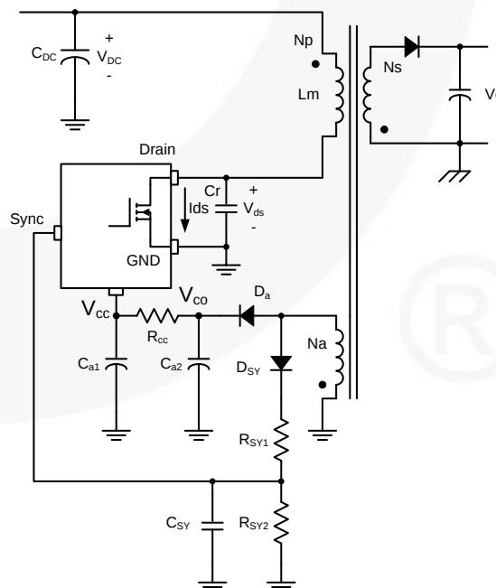
Figure 27. Synchronization Circuit
