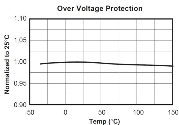
Figure 11. Over-Voltage Protection
