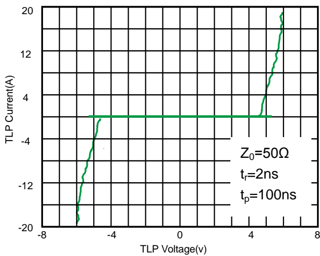
Fig 7. TLP Measurement
