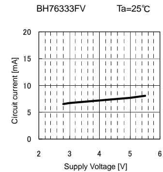
Fig.63 ICC1 vs. Supply Voltage
