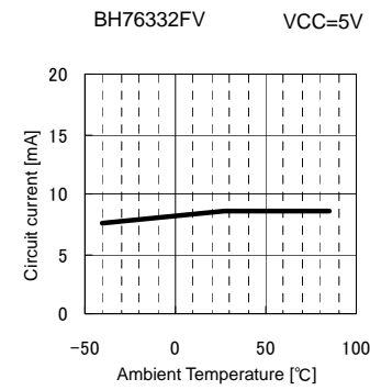
Fig.62 ICC1 vs. Ambient Temperature
