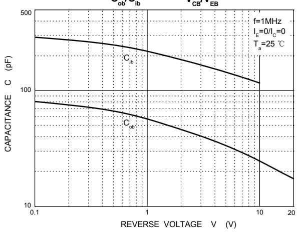
C_{ob}/C_{ib} — V_{CB}/V_{EB}
