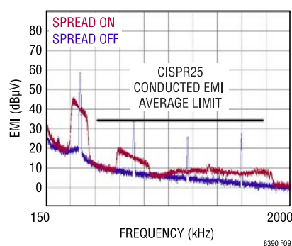
Figure 9. Average Conducted EMI Comparison
