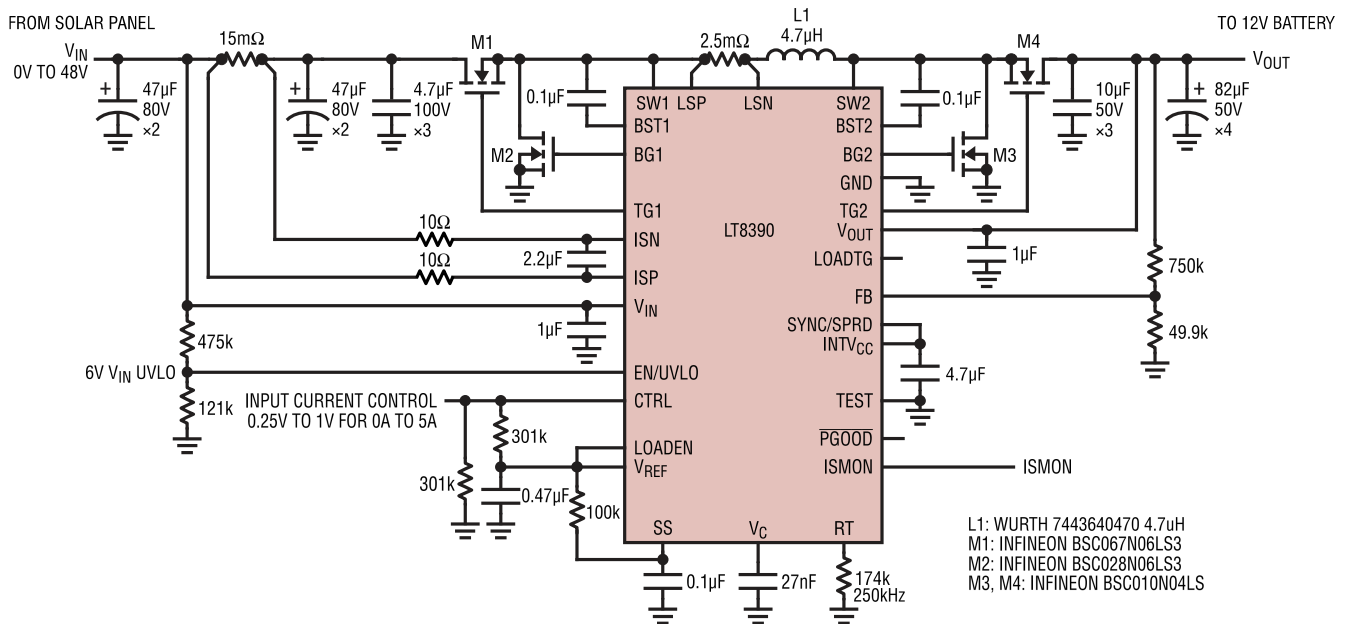
125W (25V 5A) Solar Panel to 12V Battery Charger
