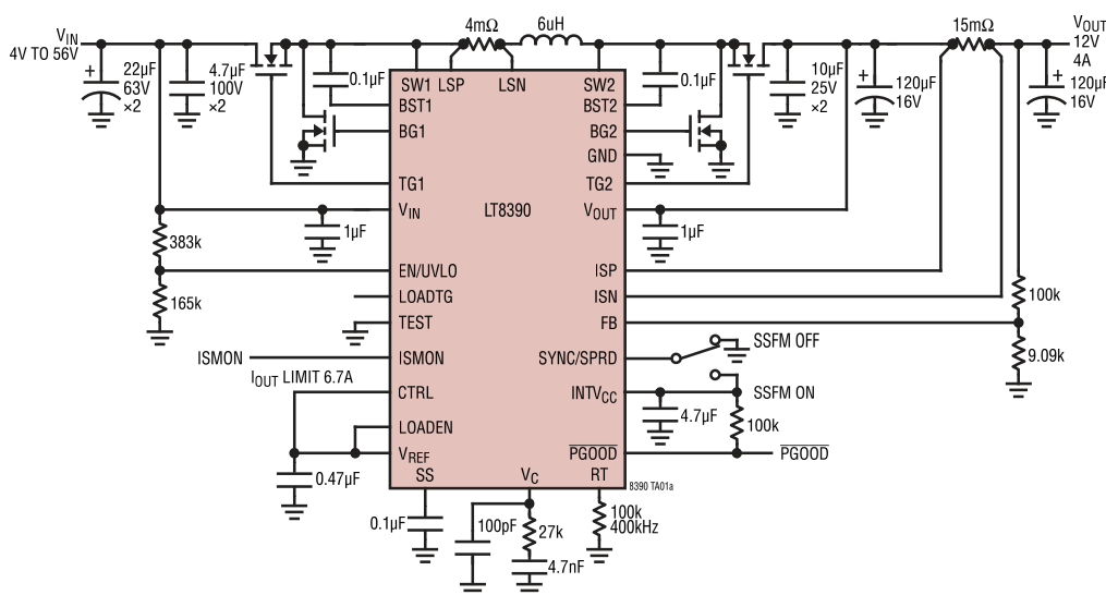
98% Efficient 48W (12V 4A) Miniature Buck-Boost Voltage Regulator
