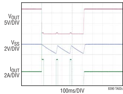
Output Short Protection ( V_{IN} = 12V , I_{OUT} = 3A )
