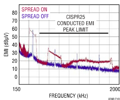
Figure 10. Peak Conducted EMI Comparison
