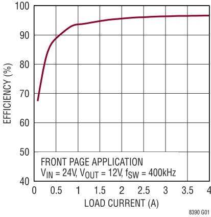
Efficiency vs Load Current (Buck Region)
