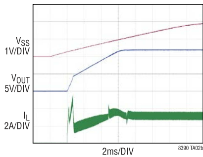
Soft Start ( V_{IN} = 12V , I_{OUT} = 3A )
