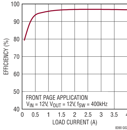
Efficiency vs Load Current (Buck-Boost Region)
