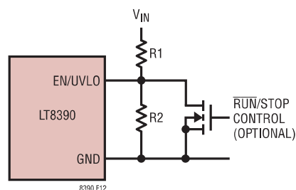
Figure 12. V IN Undervoltage Lockout (UVLO)
