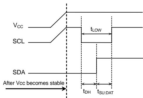
Figure 60. When SCL= 'H' and SDA= 'L'
