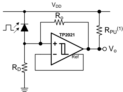
Figure 7. IR Receiver
