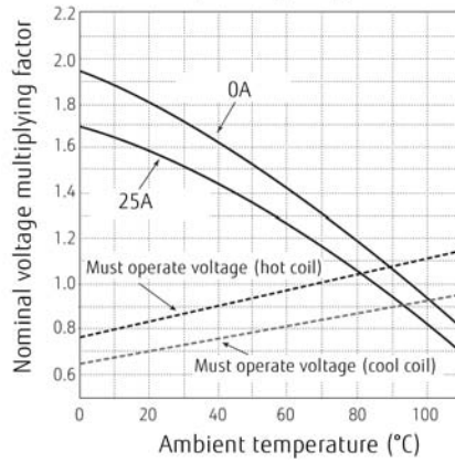
Operating range
