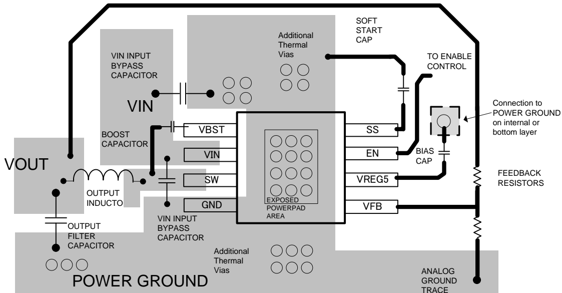
Figure 18. PCB Layout
