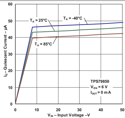
Figure 9. Quiescent Current vs Input Voltage
