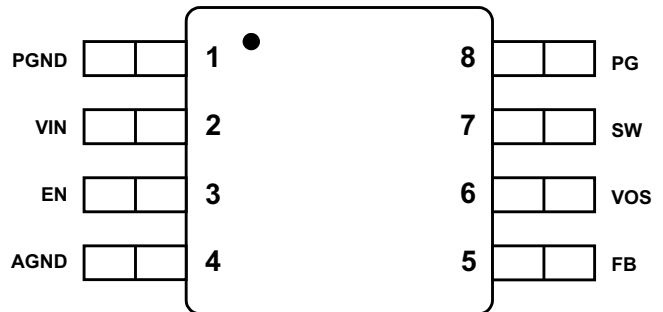
DGK Package 8-Pin VSSOP Top View
