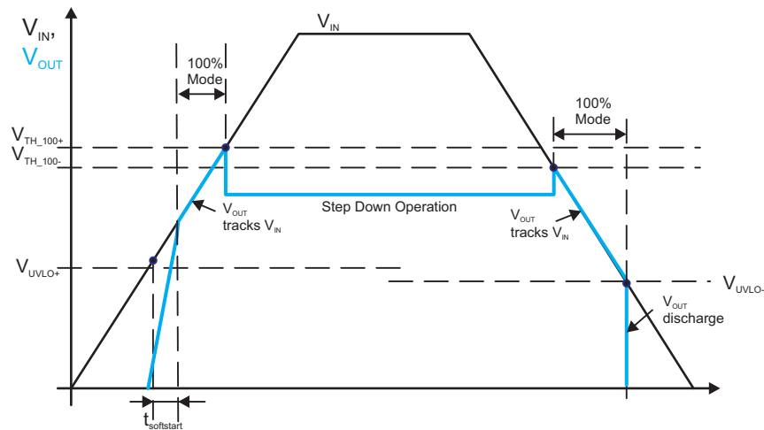
图 5. Automatic Transition into 100% Mode
