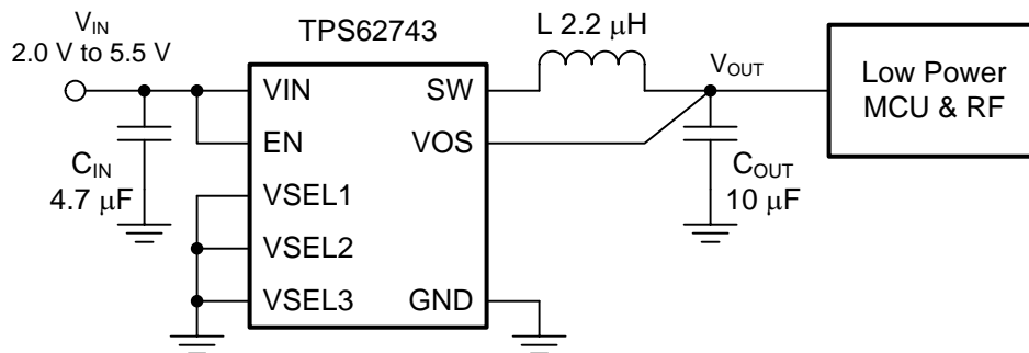
图 6. TPS62743 Typical Application Circuit
