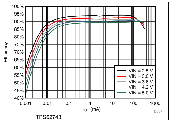
图 9. Efficiency vs Load Current; V_{OUT} = 2.1\text{ V}
