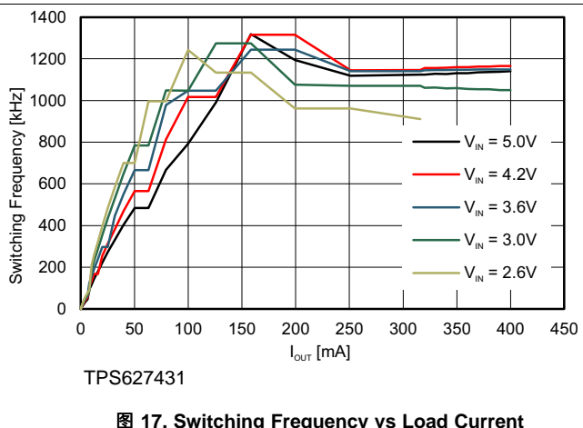
图 17. Switching Frequency vs Load Current V_{OUT} = 1.4\text{ V}
