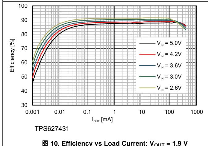
图 10. Efficiency vs Load Current; V_{OUT} = 1.9\text{ V}
