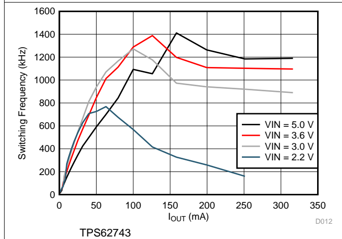
图 16. Switching Frequency vs Load Current V_{OUT} = 1.8\text{ V}
