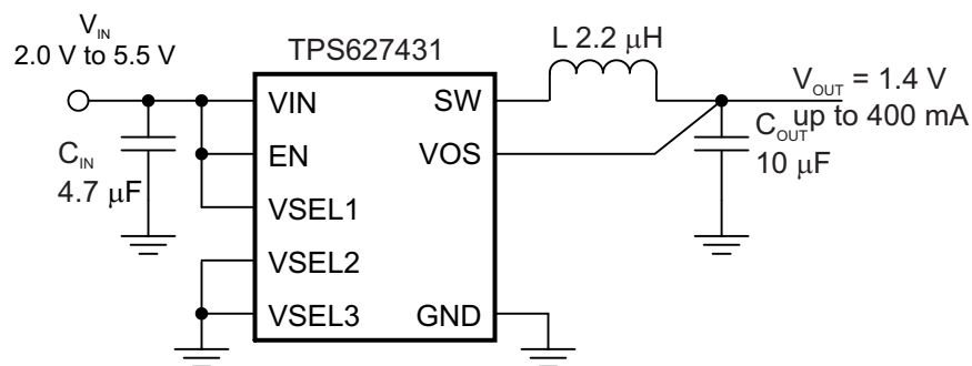
图 7. TPS627431 Typical Application Circuit
