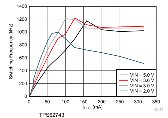
图 18. Switching Frequency vs Load Current V_{OUT} = 1.2\text{ V}
