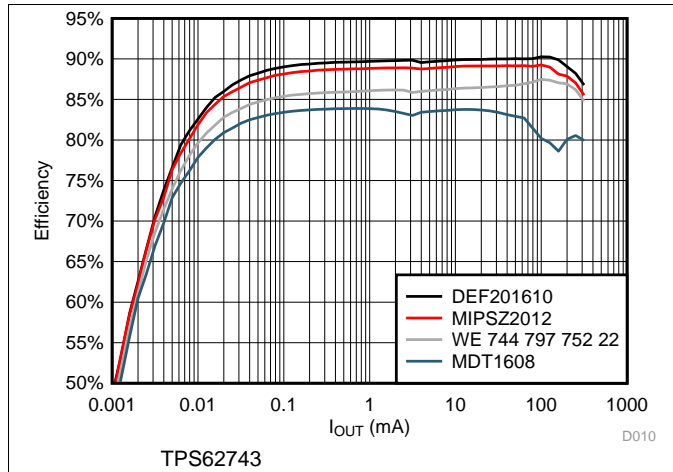
图 14. Efficiency vs Load Current; V_{OUT} = 1.8\text{ V}
