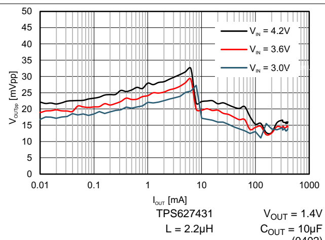
图 19. Typical Output Ripple Voltage V_{OUT} = 1.4\text{ V}
