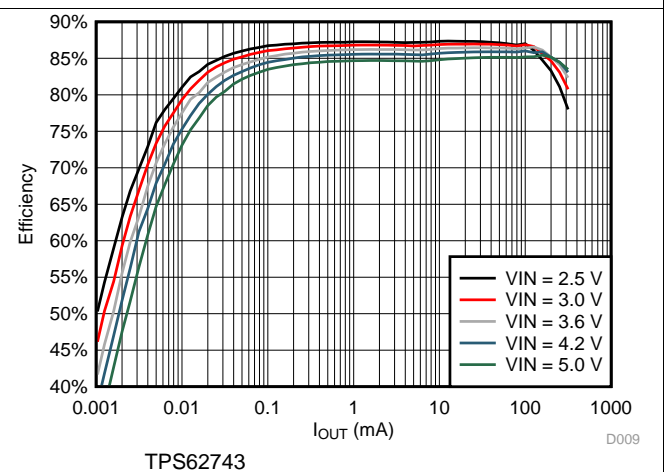
图 13. Efficiency vs Load Current; V_{OUT} = 1.2\text{ V}
