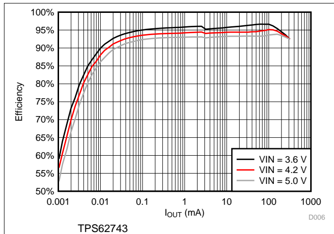
图 8. Efficiency vs Load Current, V_{OUT} = 3.3\text{ V}
