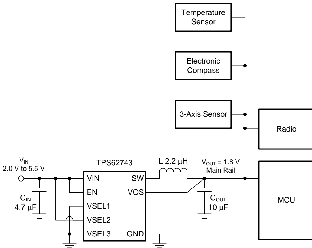
图 27. Example Of Implementation In A Master MCU Based System
