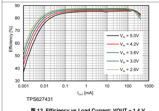
图 12. Efficiency vs Load Current; V_{OUT} = 1.4\text{ V}
