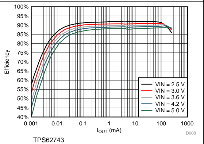
图 11. Efficiency vs Load Current; V_{OUT} = 1.8\text{ V}
