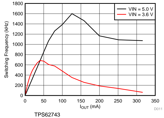
图 15. Switching Frequency vs Load Current V_{OUT} = 3.3\text{ V}
