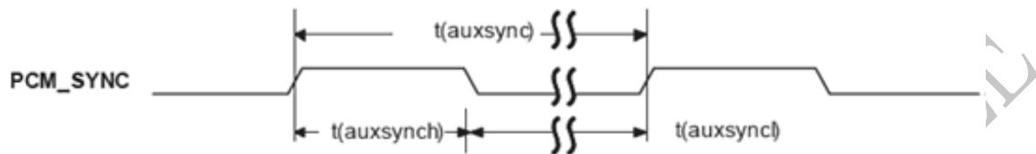
Figure 17: PCM_SYNC timing
