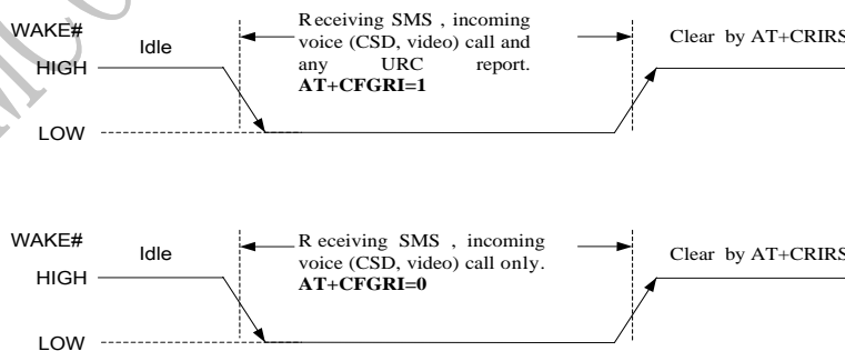
Figure 7: WAKE# behaviour
