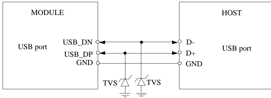
Figure 10: USB Reference Circuit
