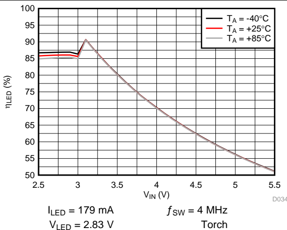
Figure 50. LED Efficiency vs Input Voltage
