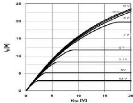
Figure 6. Output Characteristics@125°C
