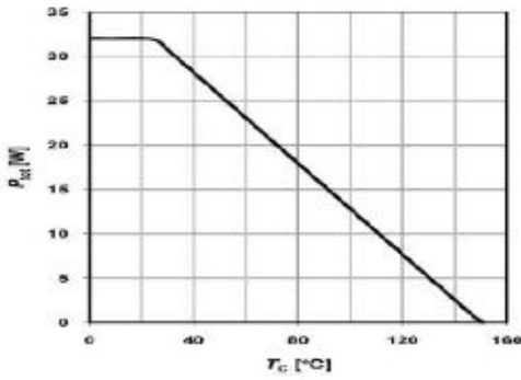
Figure 1. Power Dissipation
