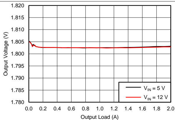
Figure 3. BUCK1, PSM Mode, Load Regulation
