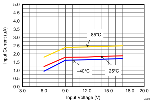
Figure 2. Shutdown Current
