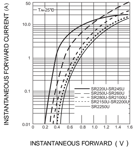
FIG.2-TYPICAL FORWARD CHARACTERISTICS
