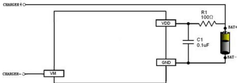
Fig 6 XB3306G in a Typical Battery Protection Circuit
