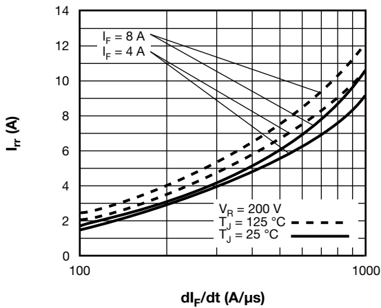
Fig. 6 - Typical Recovery Current vs. di/dt
