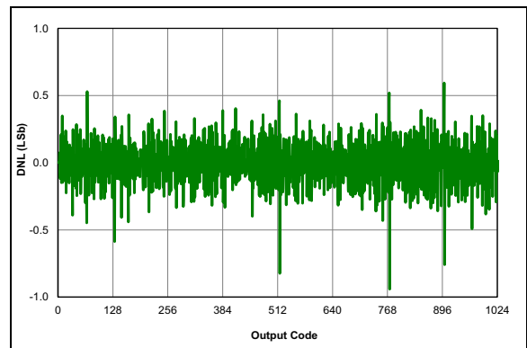
FIGURE 36-66: ADC 10-bit Mode, Single-Ended DNL, V_{DD} = 3.0V , T_{AD} = 4\ \mu S , 25^\circ C .
