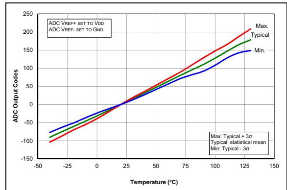
FIGURE 36-77: Temp. Indicator Slope Normalized to 20°C, High Range, V_{DD} = 3.0V , PIC16F1614/8 Only.
