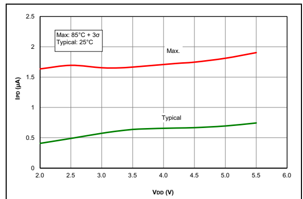
FIGURE 36-24: I_{PD} , Watchdog Timer (WDT), PIC16F1614/8 Only.
