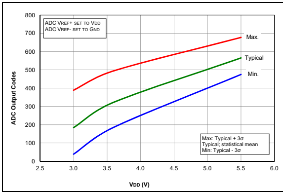
FIGURE 36-73: Temp. Indicator Initial Offset, High Range, Temp. = 20°C, PIC16F1614/8 Only.
