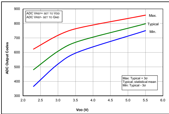
FIGURE 36-74: Temp. Indicator Initial Offset, Low Range, Temp. = 20°C, PIC16F1614/8 Only.
