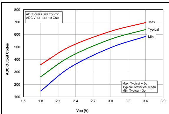
FIGURE 36-75: Temp. Indicator Initial Offset, Low Range, Temp. = 20°C, PIC16LF1614/8 Only.
