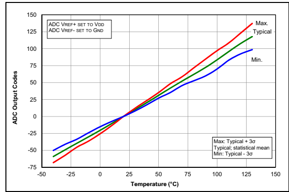
FIGURE 36-76: Temp. Indicator Slope Normalized to 20°C, High Range, V_{DD} = 5.5V , PIC16F1614/8 Only.
