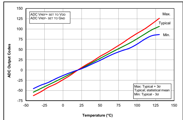
FIGURE 36-78: Temp. Indicator Slope Normalized to 20°C, Low Range, V_{DD} = 3.0V , PIC16F1614/8 Only.
