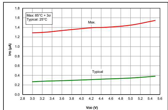
FIGURE 36-30: I_{PD} , LP Brown-Out Reset (LPBOR = 0), PIC16F1614/8 Only.
