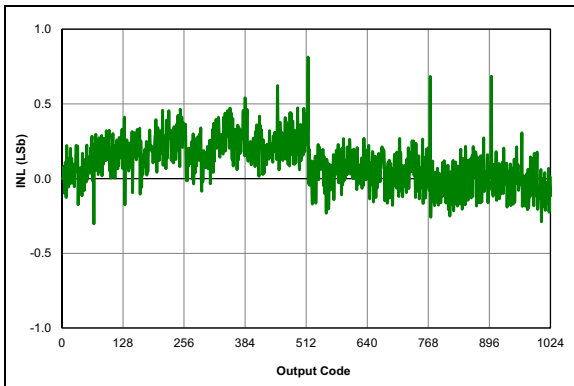
FIGURE 36-68: ADC 10-bit Mode, Single-Ended INL, V_{DD} = 3.0V , T_{AD} = 4\ \mu\text{s} , 25^\circ\text{C} .
