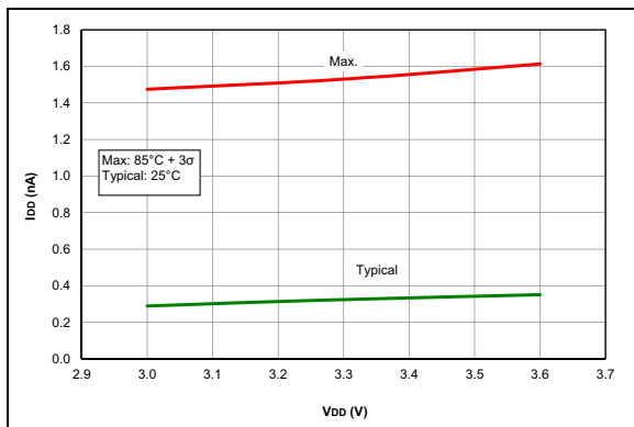
FIGURE 35-41: I_{D0} , LP Brown-out Reset (LPBOR = 0), PIC16LF1713/6 Only.
