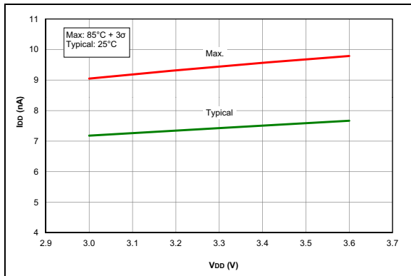
FIGURE 35-39: I_{D0} , Brown-out Reset (BOR), BORV = 1, PIC16LF1713/6 Only.
