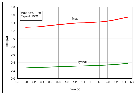
FIGURE 35-42: I_{D0} , LP Brown-out Reset (LPBOR = 0), PIC16F1713/6 Only.
