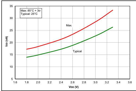
FIGURE 35-37: I_{D0} , Fixed Voltage Reference (FVR), PIC16LF1713/6 Only.
