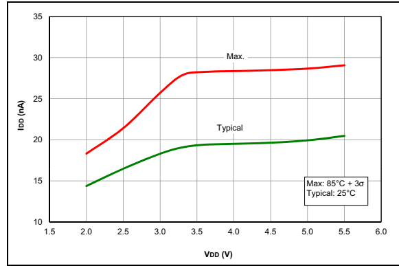
FIGURE 35-38: I_{D0} , Fixed Voltage Reference (FVR), PIC16F1713/6 Only.
