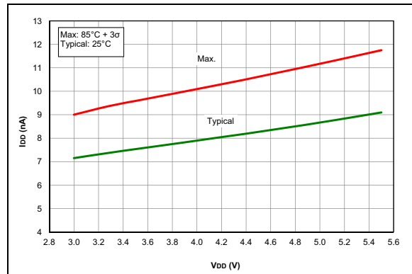
FIGURE 35-40: I_{D0} , Brown-out Reset (BOR), BORV = 1, PIC16F1713/6 Only.
