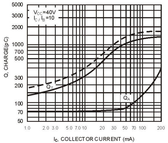
Figure 4. Charge Date
