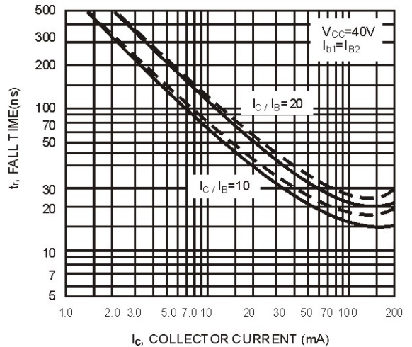
Figure 6. Fall Time
