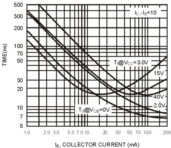
Figure 5. Turn-On Time
