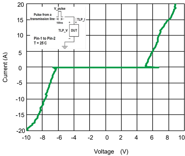
Fig 3. TLP Measurement
