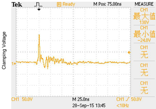
ESD clamping
