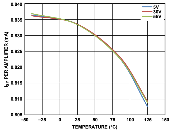
Figure 34. Supply Current ( I_{SV} ) per Amplifier vs. Temperature
