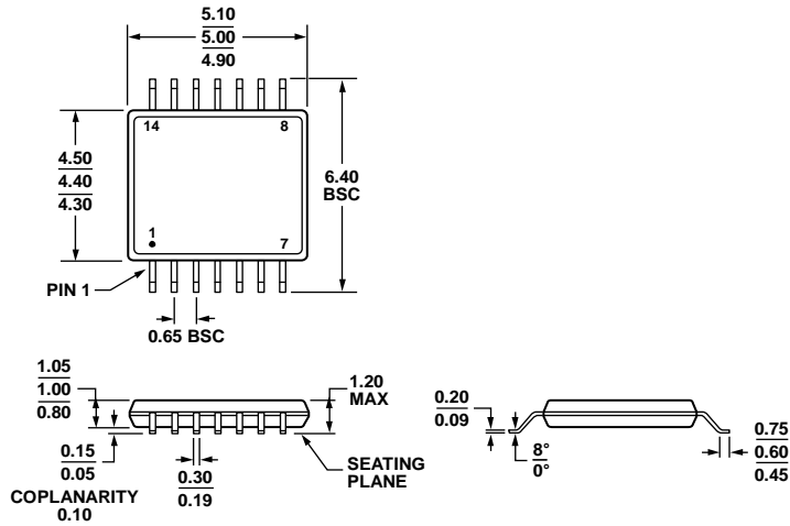
COMPLIANT TO JEDEC STANDARDS MO-153-AB-1 Figure 93. 14-Lead Thin Shrink Small Outline Package [TSSOP] (RU-14) Dimensions shown in millimeters
