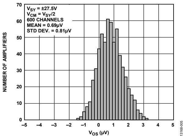
Figure 8. Input Offset Voltage Distribution, V SY = ±27.5 V
