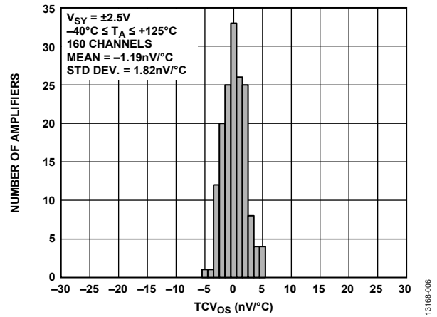
Figure 9. Input Offset Voltage Drift Distribution, V SY = ±2.5 V
