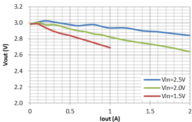
BL8531C CB5TR30 Output Voltage VS Output Current
