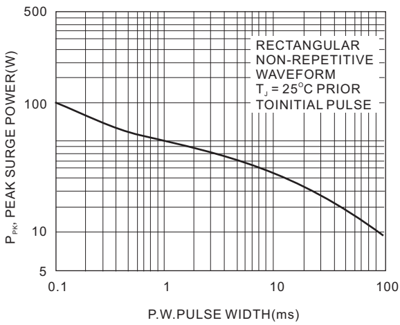
FIG. 2-MAXIMUM SURGE POWER
