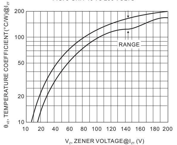
FIG. 5-UNIT 10 TO 200 VOLTS
