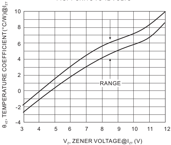
FIG. 4-UNITS TO 12 VOLTS
