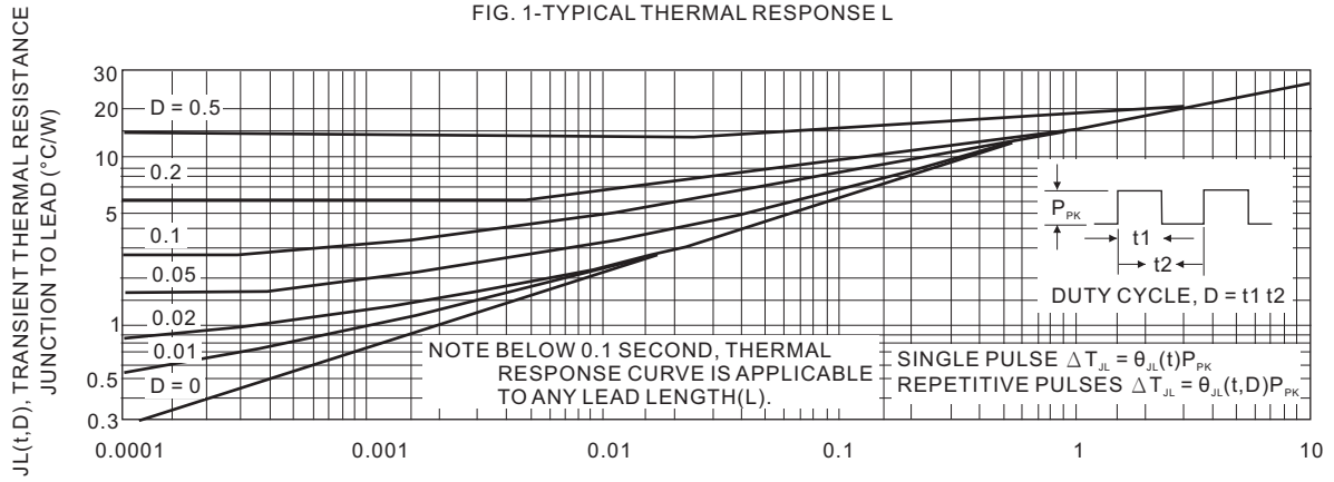
FIG. 1-TYPICAL THERMAL RESPONSE L
