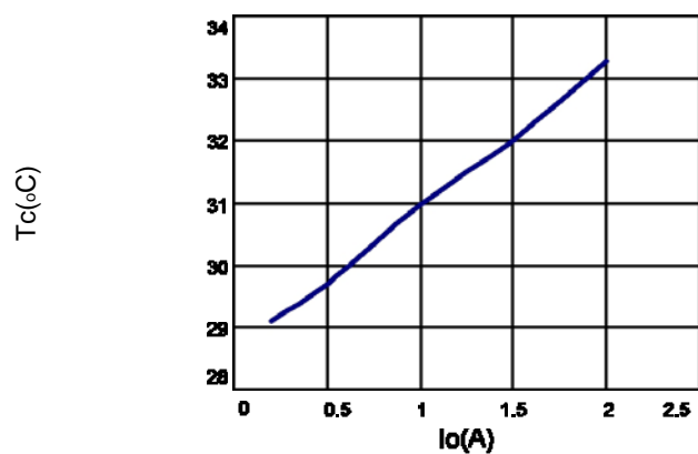
Case Temperature vs Output Current (V_{IN}=5V, V_o=1.8V, T_a=27^{\circ}C)
