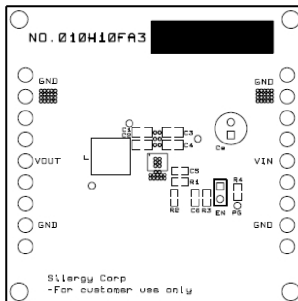
Figure 3. Top Silkscreen
