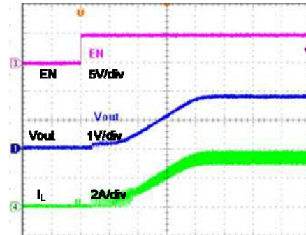
Time (200us/div)
