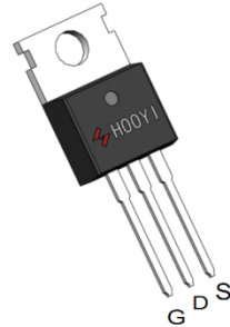
TO-220FB-3L
